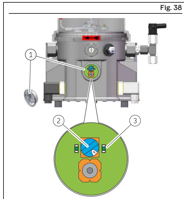
Control circuit board for P203
