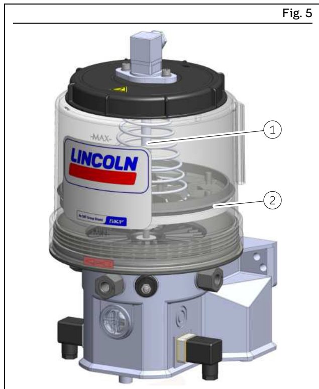
P203 with a follower plate
