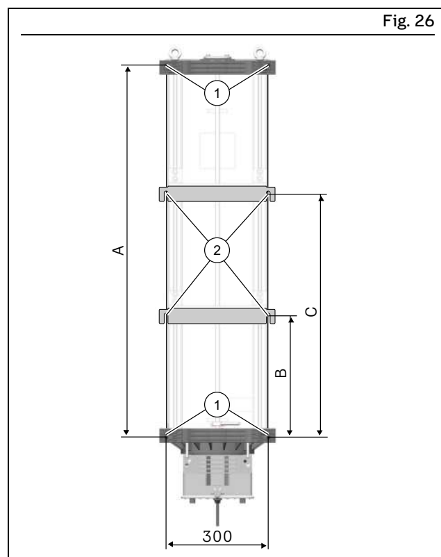
Assembly holes P203 with Xx_G- / XBxG reservoir
