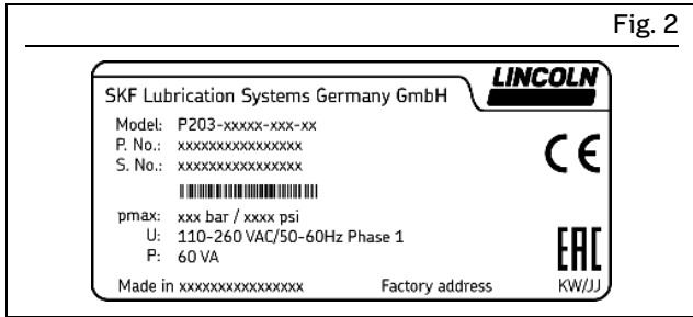
VAC type plate
